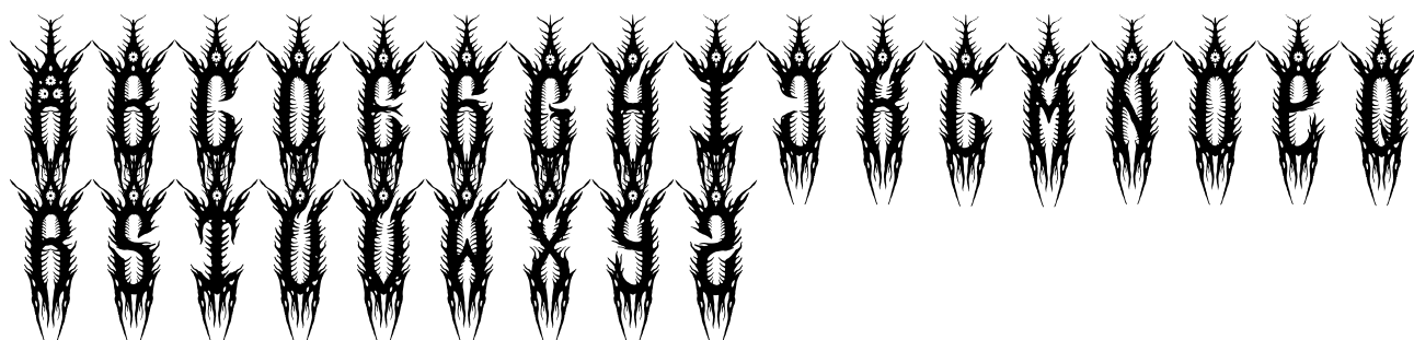
Lowercase Characters
